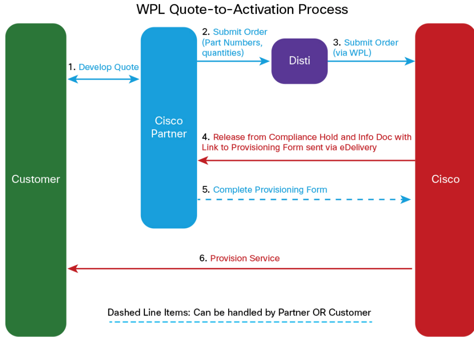
Figure 4. High-Level Summary of a WPL Transaction
