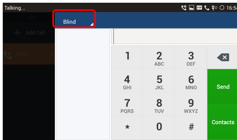
Figure 58: Blind Transfer
